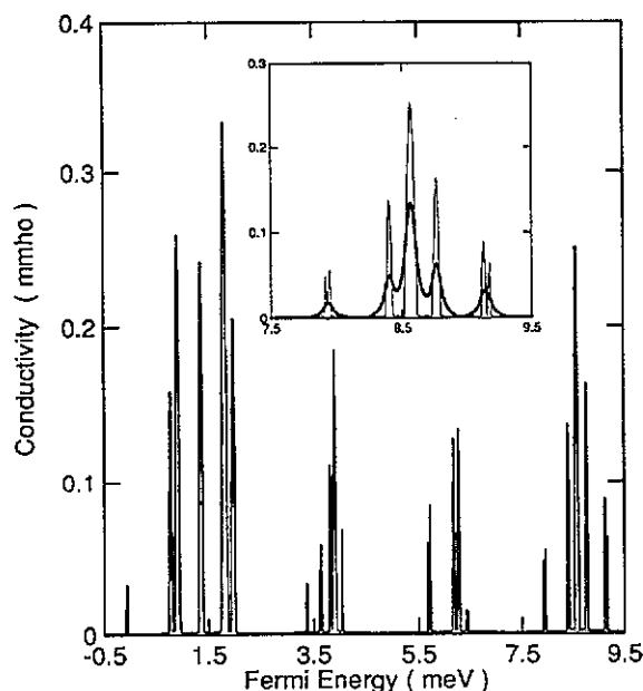
Figure 3. Band conductivity showing splitting of the lowest Landau level for B = 1.4 T, p/q = \frac{7}{2} . The inset shows in more detail the splitting of one of the Landau levels, calculated without any smoothing, and (bold line) smoothed by a Lorentzian corresponding to an inelastic scattering time of 10 ps.
