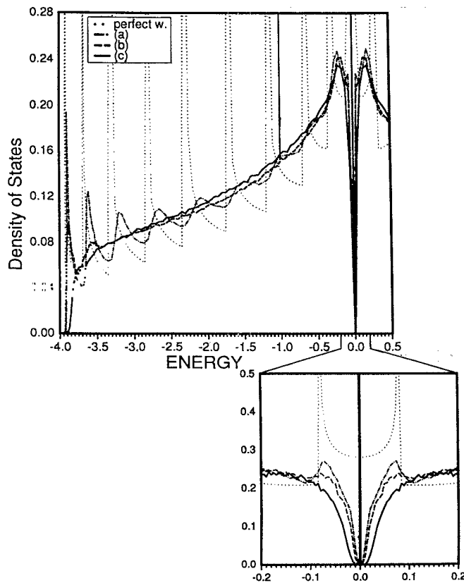
FIG. 4. The density of states (per site, per unit energy) for a monolayer wire, together with the perfect case (dotted line), corresponding to (a) only meandering wire; (b) wire in Fig. 1(b); (c) wire in Fig. 1(c). The lower diagram shows the region around energy E = 0 in more detail.
