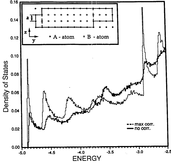
FIG. 6. The density of states (per site, per unit energy) for the two-layer wire, where each layer has a constant width and no islands, only the center of wire is fluctuating (meandering wire), for no correlation (full line) and maximum correlation (broken line) between the layers. The inset figure shows a cross section of the two-layer wire (not with maximum correlation between layers). Broken lines represent the effective size of the cross section for long-wavelength electrons.
