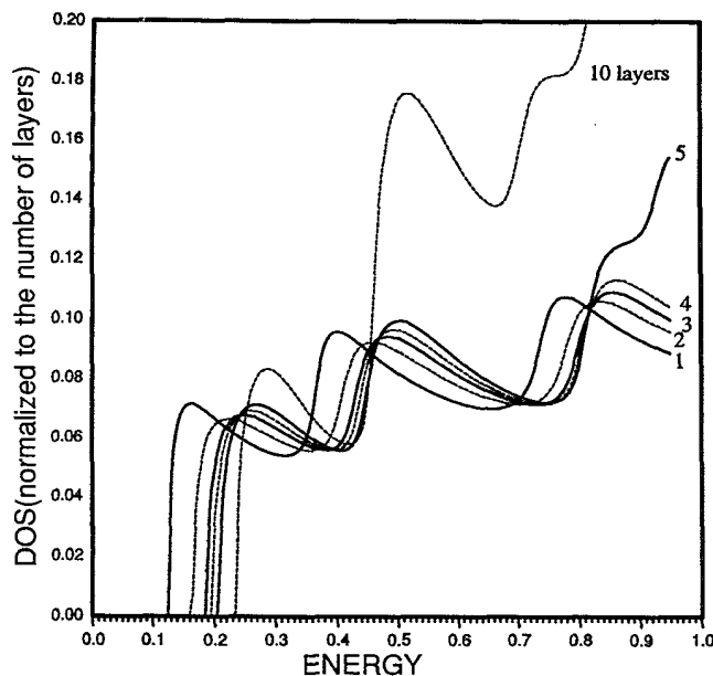
FIG. 3. The density of states (per site, per unit energy) multiplied by the number of layers in the wire, for the cases of one, two, three, four, five, and ten layers in the wire. The origin of the band is shifted to 0 in each case. The energy is in units of V .
