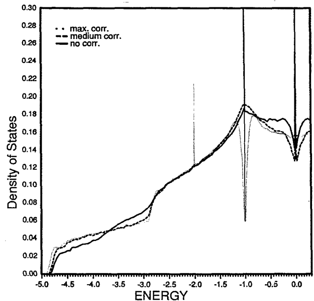
FIG. 5. The density of states (per site, per unit energy) for the two-layer real wire with islands, for zero correlation (full line), medium correlation (broken line), and maximum correlation (dotted line) between the layers. A section of a layer is given in Fig. 1(c).
