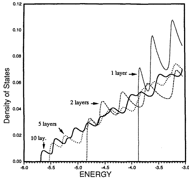
FIG. 2. The density of states (number of eigenvalues per site, per unit energy) for a one-, two-, five-, and ten-layer perfect wire with island concentration p = 5\% , calculated using the CPA. The energy E is expressed in terms of the off-diagonal H matrix elements V .
