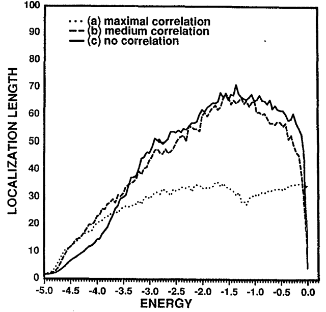
FIG. 10. As in Fig. 9, but for a wire with islands.
