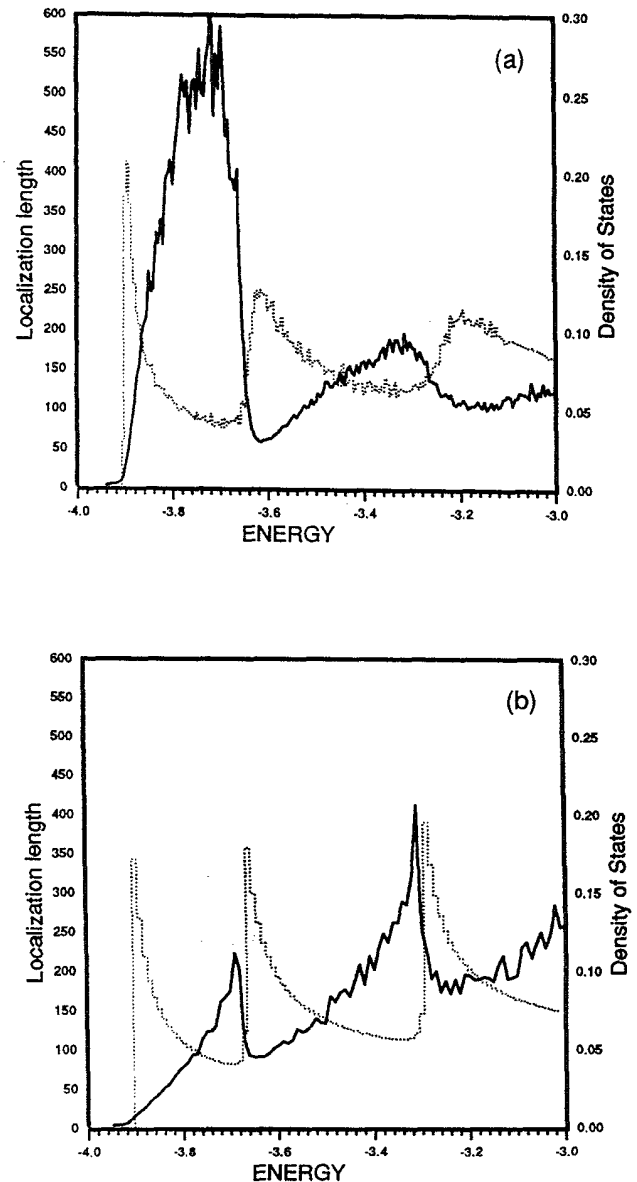
FIG. 8. The localization length (full line) and the density of states (dotted line) for energies near the band edge for a monolayer: (a) meandering wire (width of each slice is constant and equal to ten lattice spacings, no islands, only center of wire is fluctuating), and (b) a perfect wire with islands, concentration of islands p = 1\% .
