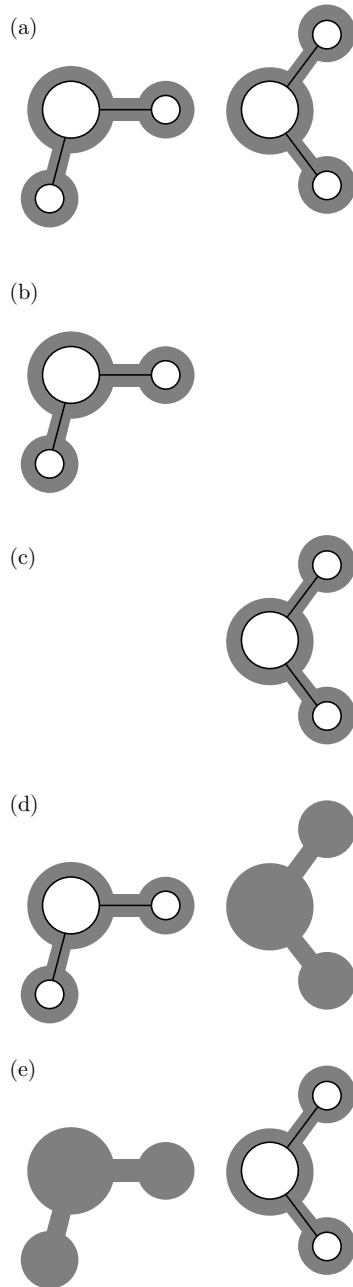
Fig. 1. Basis set superposition error occurs in the calculation of the binding energy of the dimer shown in (a) when the molecular energies are calculated as in (b) and (c) with only the basis functions (in grey) of the atoms (white disks) associated with the individual molecule. The counterpoise correction calculates the molecular energies as in (d) and (e) with the same basis set as for the dimer (a).
