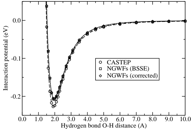
Fig. 5. Interaction potential of a water dimer obtained using a minimal basis set of fully optimised orbitals (NGWFs)
