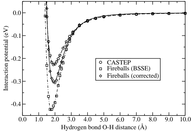
Fig. 3. Interaction potential of a water dimer obtained using a minimal basis set of fireballs
