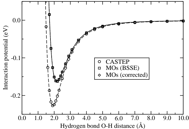
Fig. 4. Interaction potential of a water dimer obtained using a minimal basis set of local orbitals pre-optimised for isolated water molecules (MOs)
