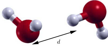
Fig. 2. Water dimer geometry showing the hydrogen bond O-H distance d .
