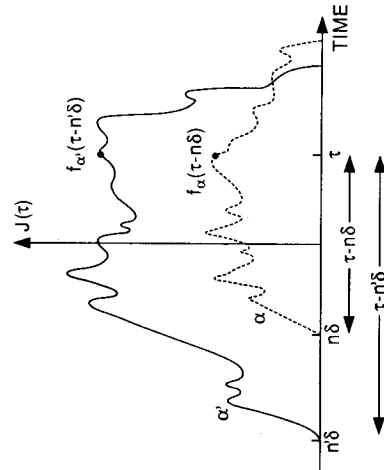
Fig. 6. Linear superposition of avalanches.
