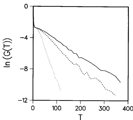
FIG. 1. Semilog plot of the distribution function G(T) defined in Eq. (7) for three different system sizes: dotted 20 \times 20 , dashed 50 \times 50 , and solid 75 \times 75 .
