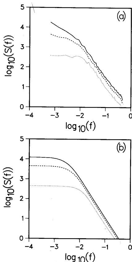
FIG. 2. (a) Power spectrum of the flow down the slope. Individual avalanche signals started at random times are superimposed linearly and the resulting time sequence is Fourier transformed. (b) Power spectrum obtained by inserting the measured G(T) from Fig. 1 into Eq. (6). The rate v is equal to 0.5. The dotted, the dashed, and the solid curves are for system size 20 \times 20 , 50 \times 50 , and 75 \times 75 , respectively.
