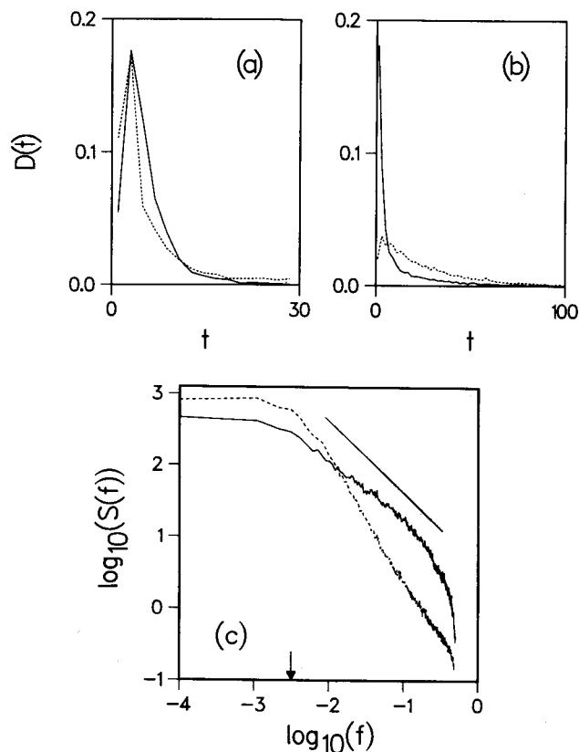
FIG. 3. Distribution of the intervals \Delta t between avalanches (dashed line) and the duration of avalanches \tau (solid line) for the flow (a) over the rim and (b) down the slope, in a continuously driven automaton. The probability for adding sand at a site is 0.05 per time step. The associated power spectra are shown in (c). Solid line corresponds to flow over the rim (the data are multiplied by 10^2 ), dashed line to flow down the slope. The straight line indicates 1/f behavior. The arrow locates the frequency 2\pi/51 —the characteristic frequency in the Lorentzian corresponding to G(T) in Fig. 1.
